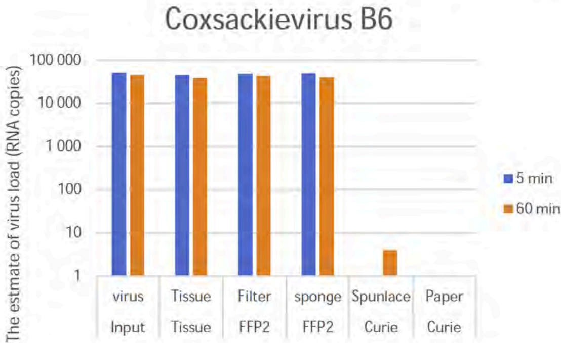
Figure 3 - Test results of the enterovirus (Coxsackievirus B6) - Virus RNA detected in buffer using RT-qPCR. For Curie Paper, 3/3 in 5min and 60min incubation times were entirely negative. At the same time, only 1/3 with Curie Spunlace had less than 10 viruses left.
